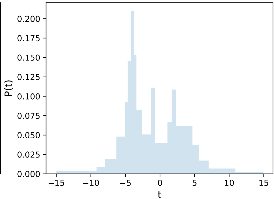
hist(t, bins="blocks")
