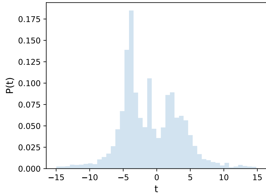
hist(t, bins="knuth")
